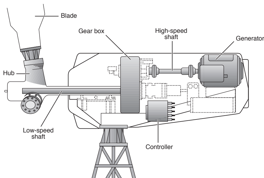
ELECTRICITY GENERATING WIND TURBINE The major components of this device are the blades, shaft, gearbox and generator. On large machines, additional controllers and drive motors ensure that the machine is positioned for optimal capture of the wind.
