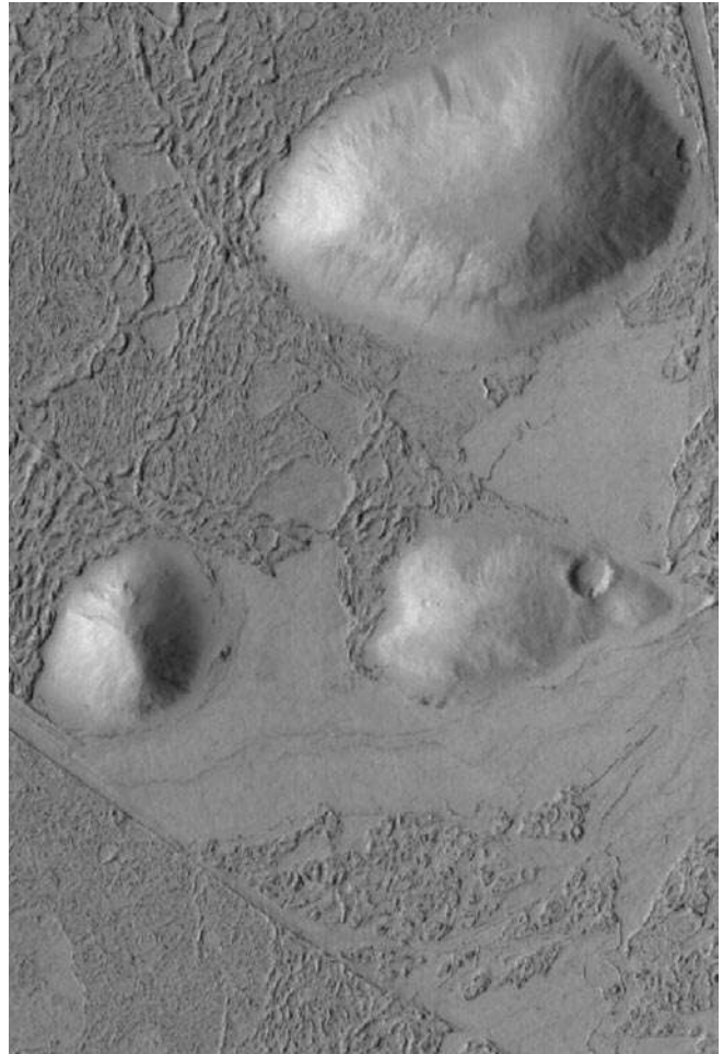
Figure S2. Degraded craters on Mars.
