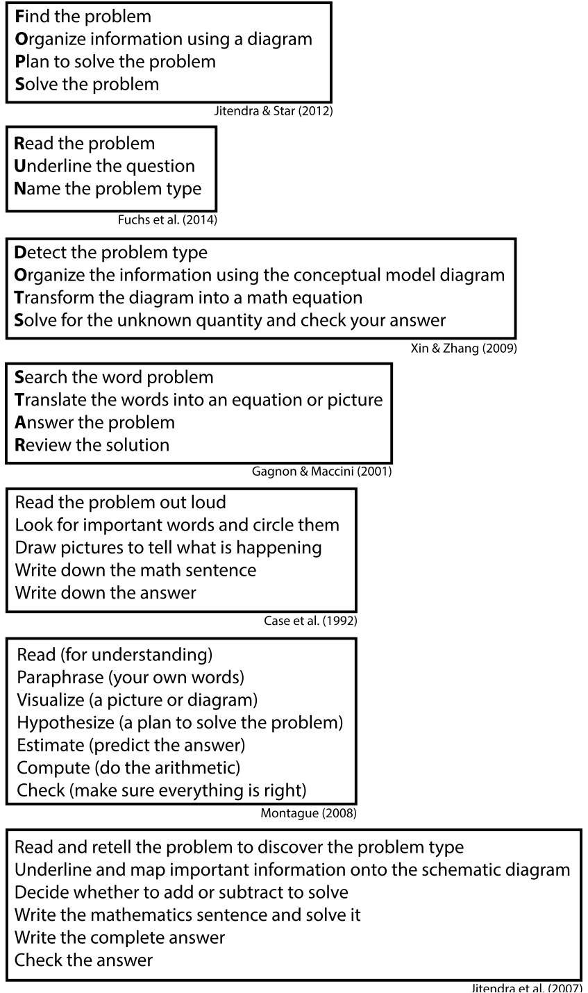
Figure 1. Sample attack strategies
