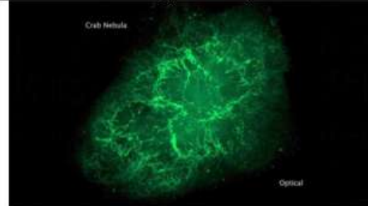
Crab Nebula at optical (visible) wavelengths
