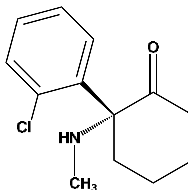
(R)-ketamine
