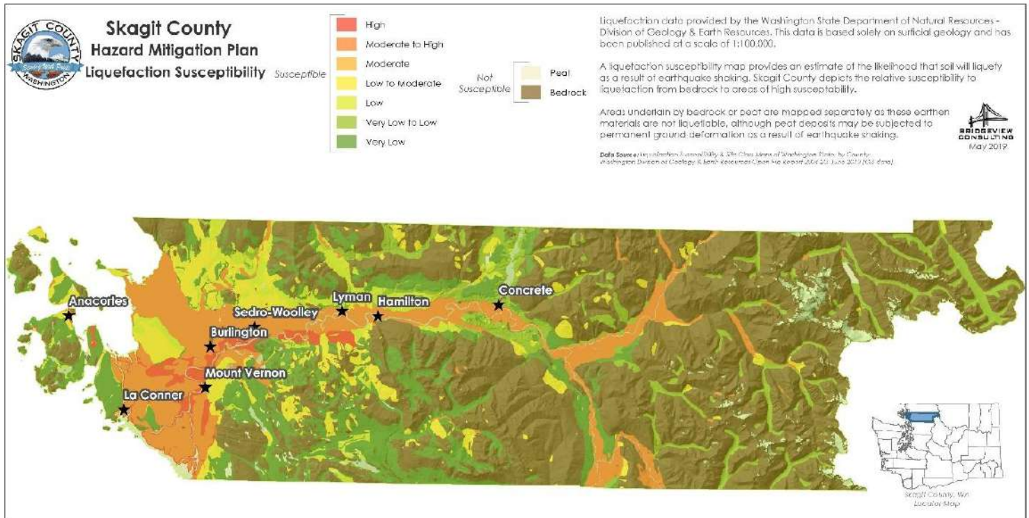
Figure 6-10 Liquefaction Susceptibility Zones
