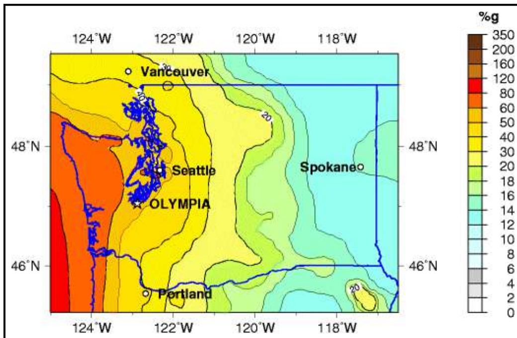
Figure 6-13 PGA with 2-Percent Probability of Exceedance in 50 Years, Northwest Region
