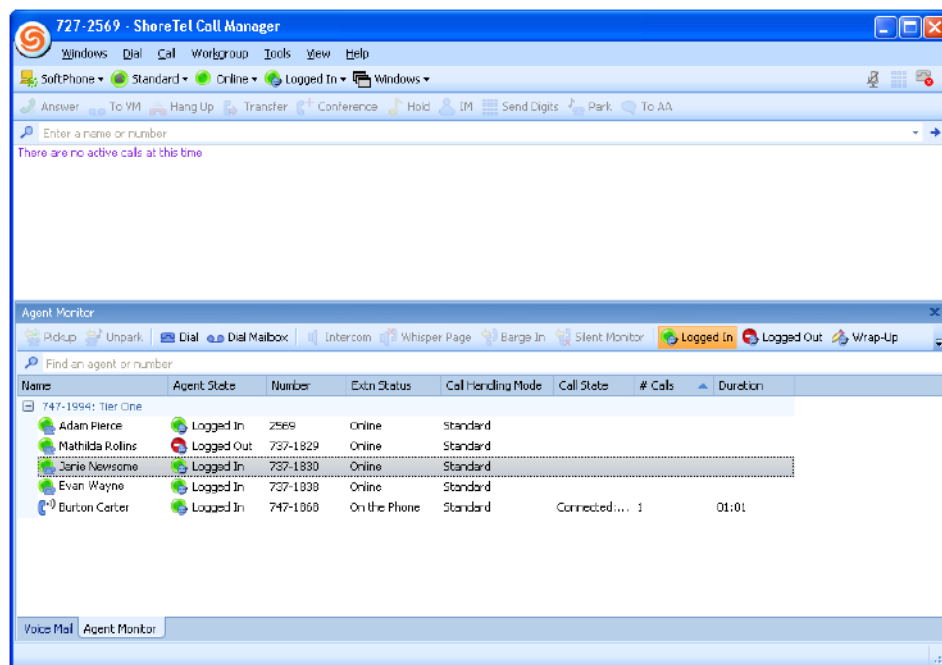
Figure 12-2 Agent Monitor
