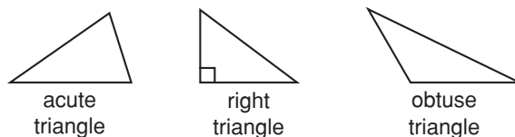
Triangles Classified by Angles
