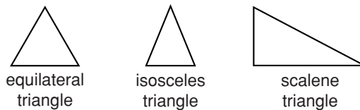
Triangles Classified by Sides
