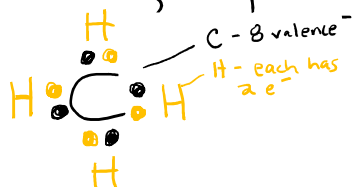
Methane, \text{CH}_4
