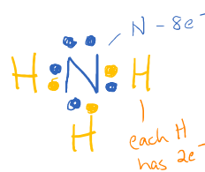
Ammonia, \text{NH}_3
