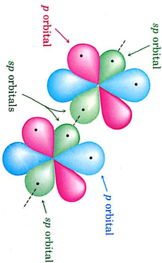
Figure 1.15 Structure of acetylene
