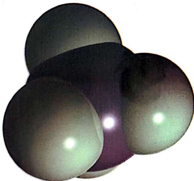
Figure 1.9 Structure of methane
