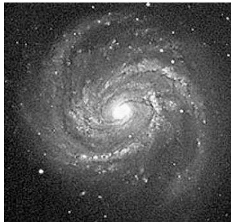
Visible - 2 (AAO)
