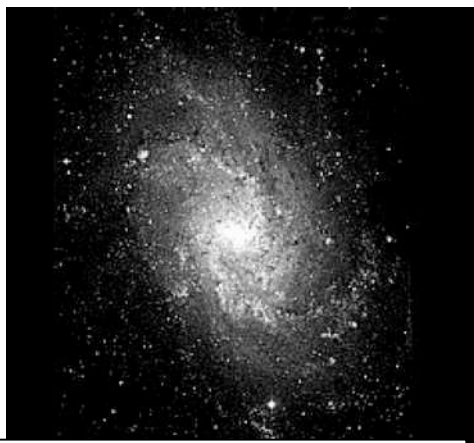
Visible - 5 (IAC/RGO/Malin)
