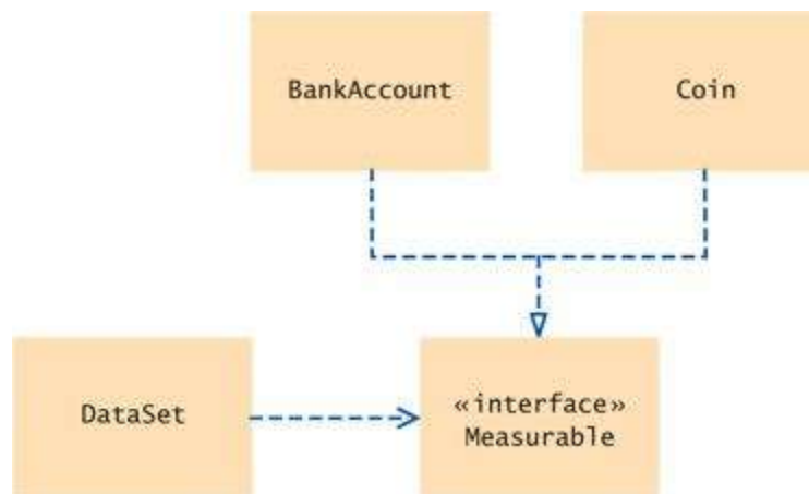
UML Diagram of the DataSet Class and the Classes that Implement the Measurable Interface
