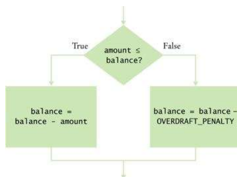
Flowchart for an if/else Statement
