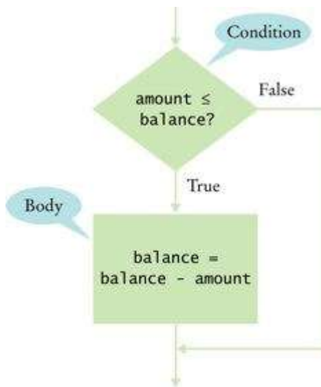
Flowchart for an if Statement
