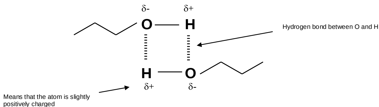
Figure 1 – Hydrogen bonding in an alkanol
