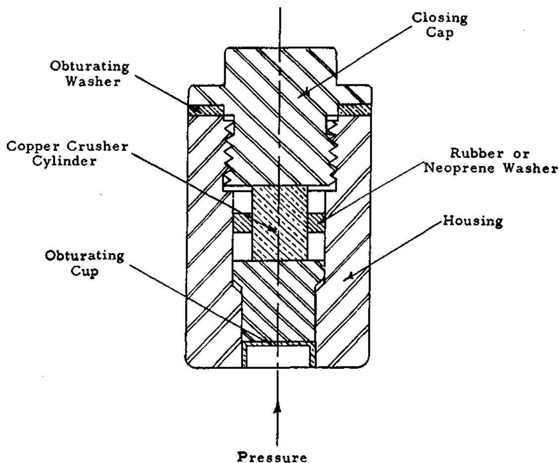
FIGURE 4-11. Cross Section of Internal Copper Crusher Pressure Gauge Using Cylindrical Copper Crusher.
