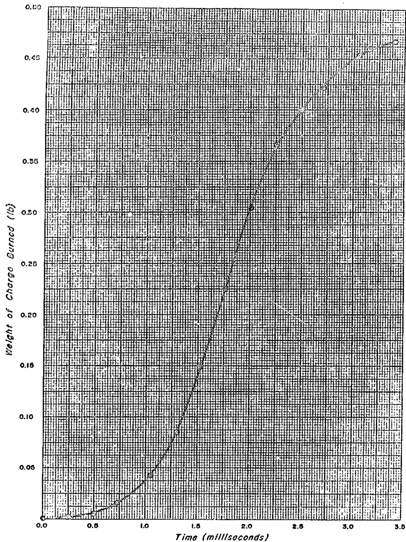
FIGURE 2-4. Charge Burned Versus Time for 37mm Gun
