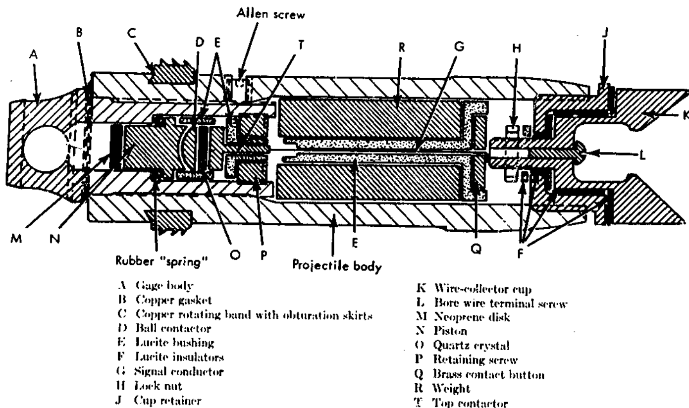
FIGURE 4-22. Diagram of Quartz Piezoelectric Base-Pressure Gauge Mounted in the Projectile.
