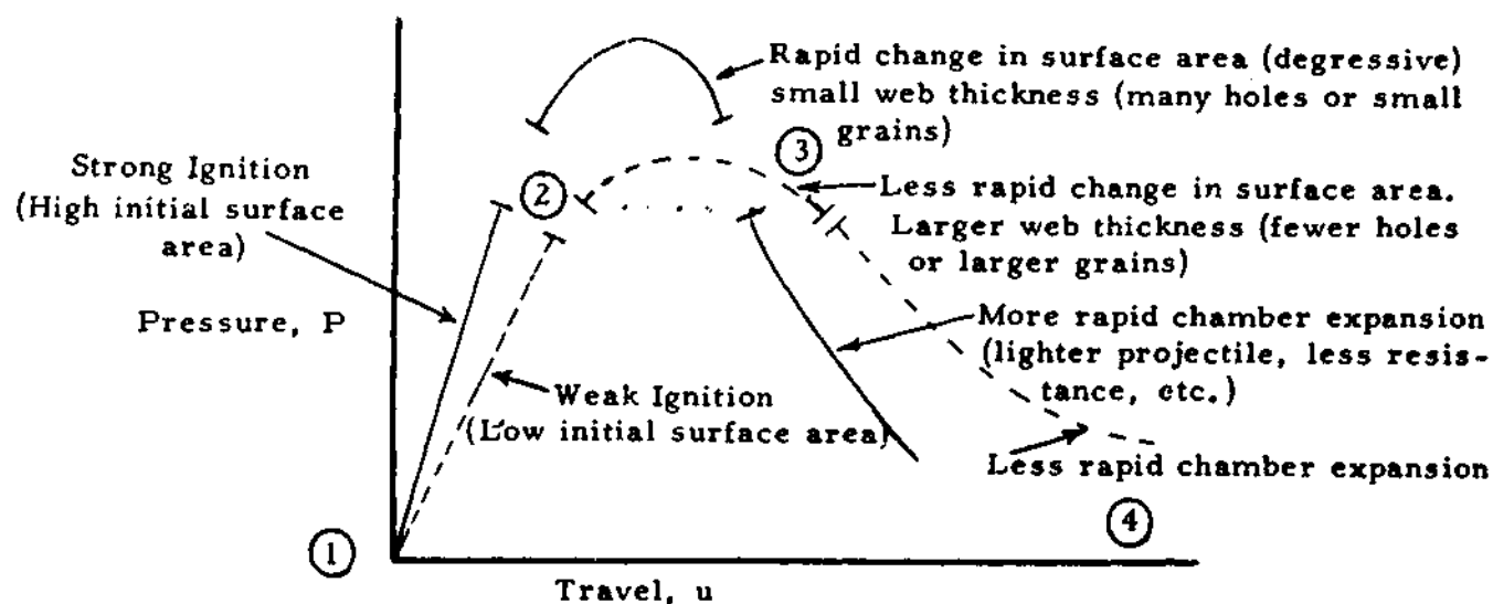
FIGURE 1-4. Pressure-Travel Relationship.
