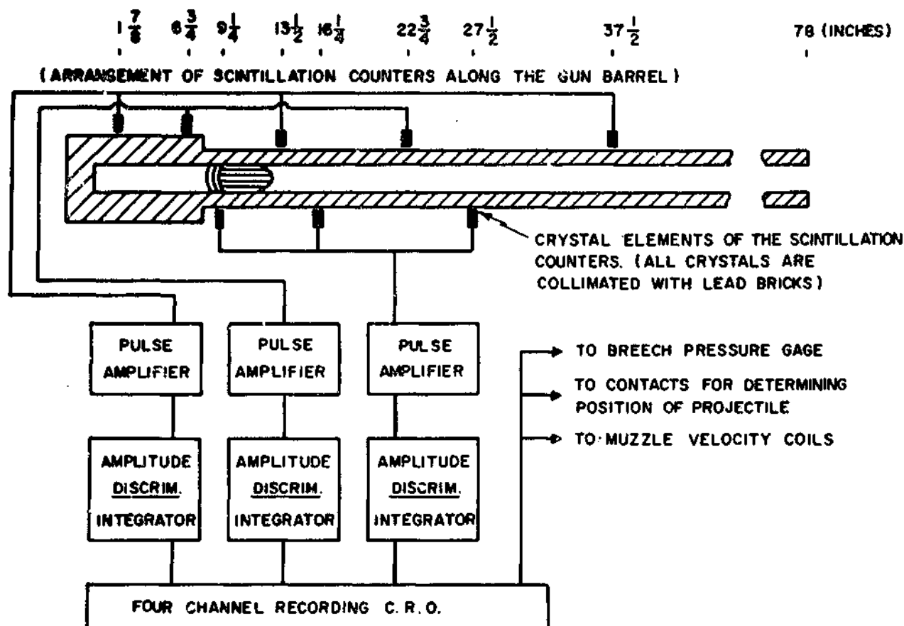
FIGURE 4-27. Block Diagram of Apparatus for Observing Motion During Firing of a Radioactive Source Embedded Initially in a Propellant Grain.
