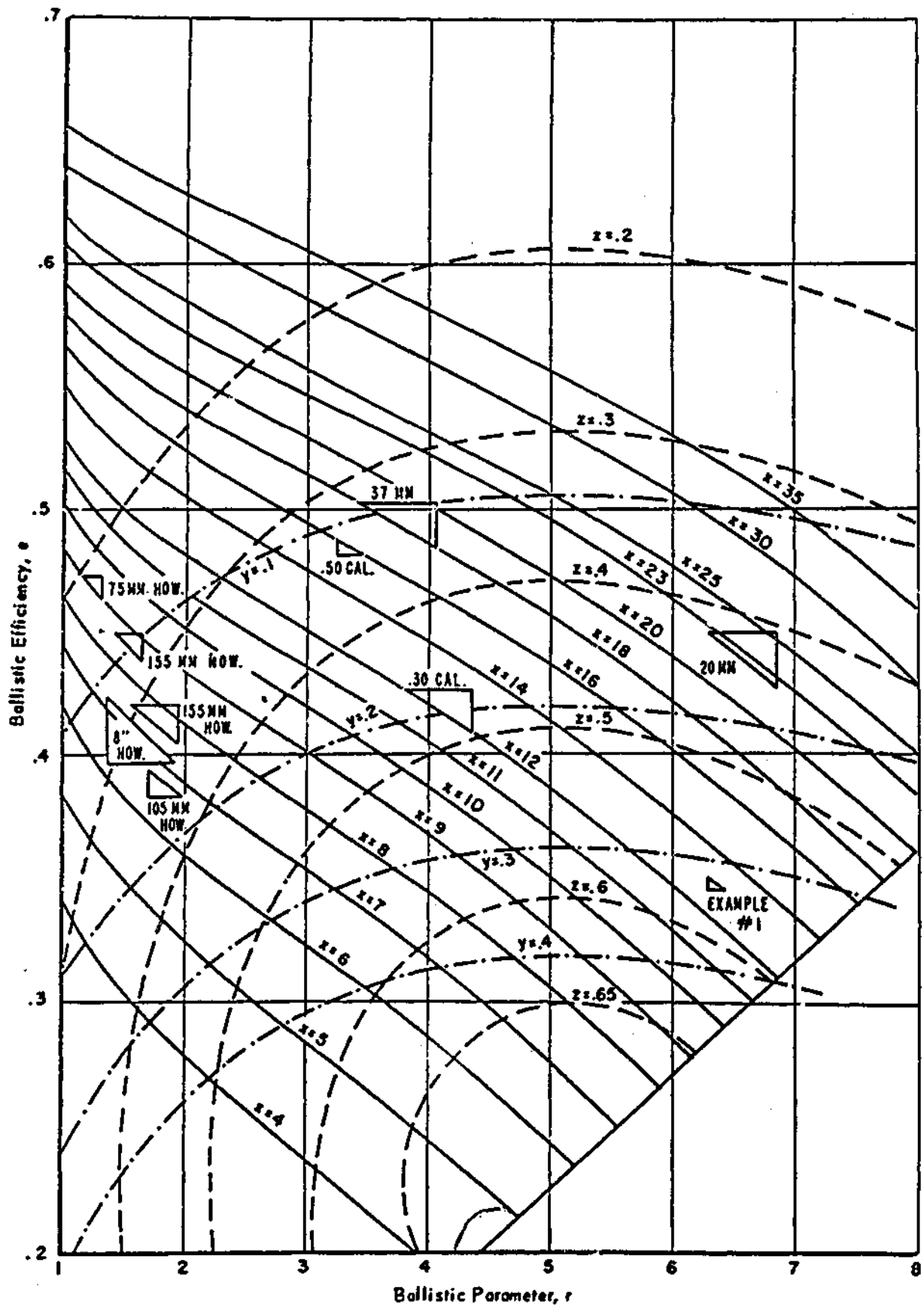
CHART 2-4. Chart for Interior Ballistic Calculations by the Scheme of Strilinatser
