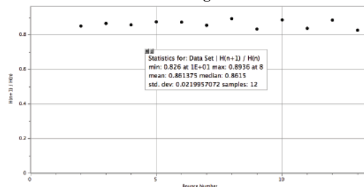
GRAPH 5: Rebound Ratio against Bounce Number
