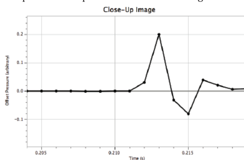
Graph 2: Close Up of Air Pressure Offset against Time
