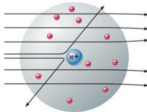
Rutherford Model 1908
