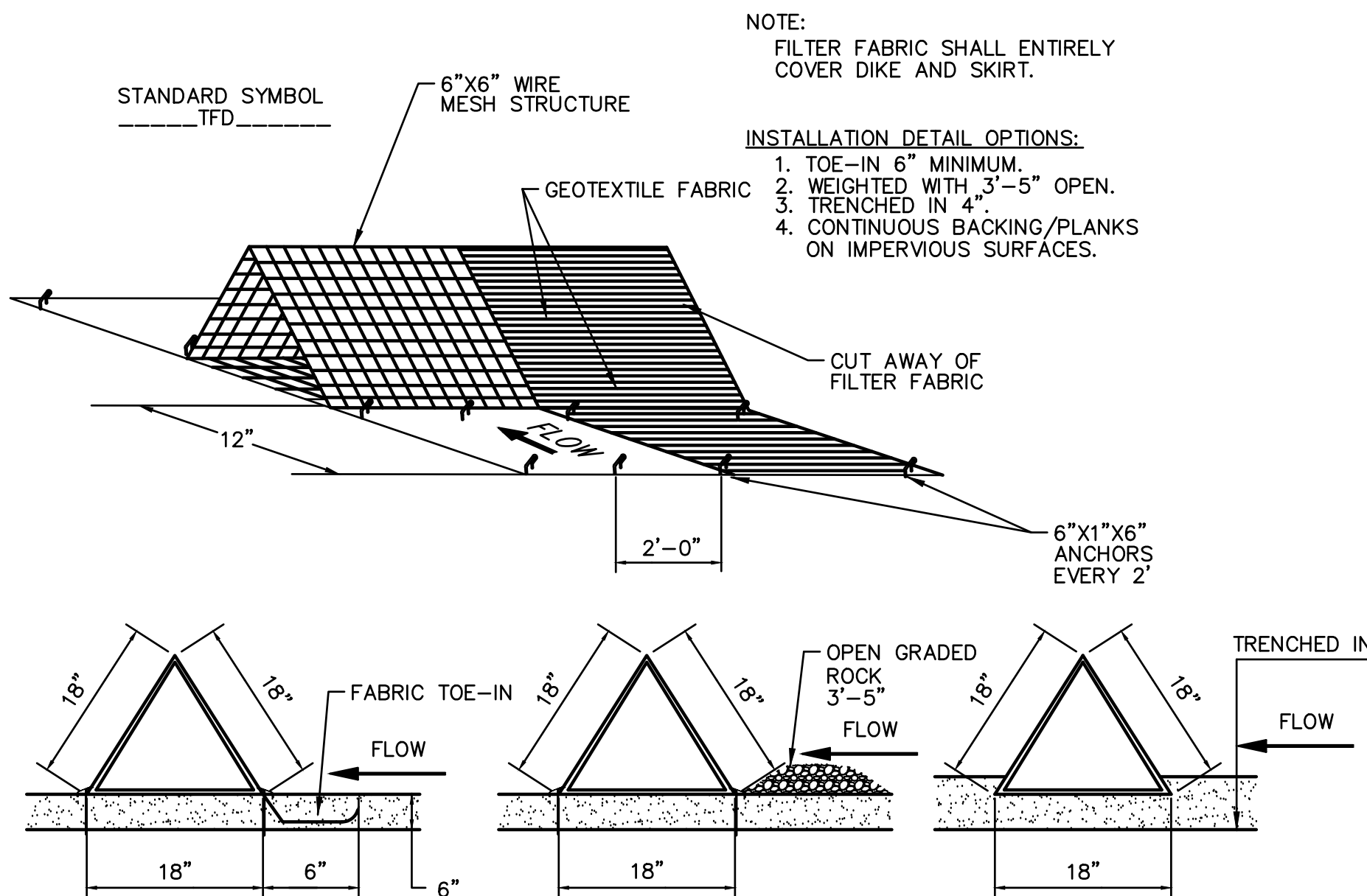
TEMPORARY CONSTRUCTION ENTRANCE NO SCALE
