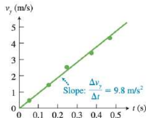
FIGURE 2.23 A velocity-versus-time graph for a falling ball.
