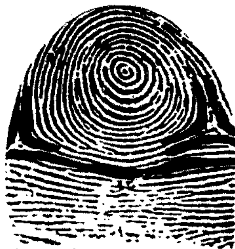
Figura 1.91. Verticilo mesodelto
