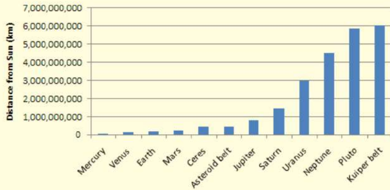
Distance of well-known solar system objects from Sun
