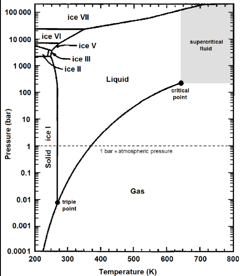
Figure F. Phase Diagram for Water
