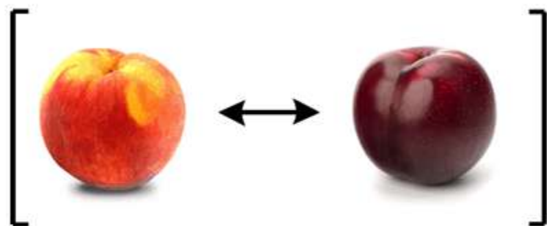
Resonance forms
