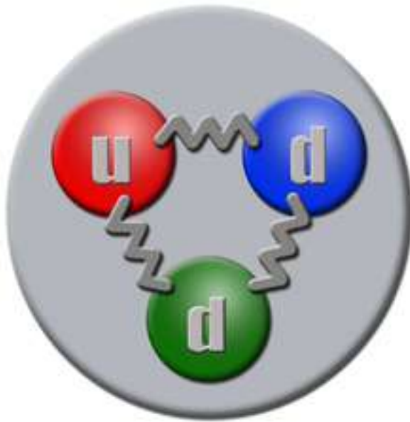
Neutron
