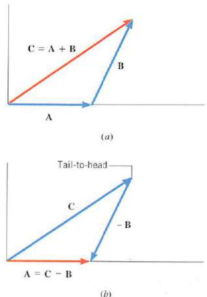
Figure 1.14 (a) Vector addition according to C = A + B . (b) Vector subtraction according to A = C - B = C + (-B) .
