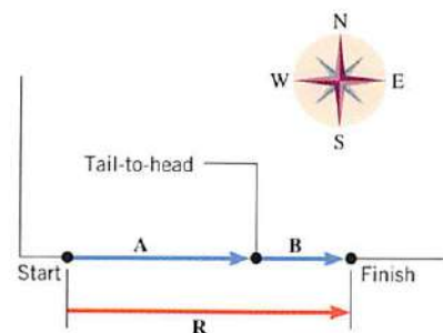
Figure 1.9 Two colinear displacement vectors A and B add to give the resultant displacement vector R .
