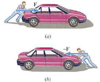
Figure 1.13 (a) The force vector for a man pushing on a car with 450 N of force in a direction due east is F . (b) The force vector for a man pushing on a car with 450 N of force in a direction due west is -F .
