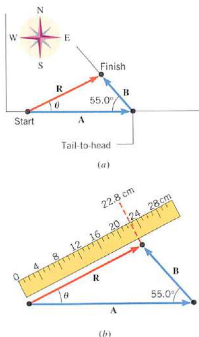
Figure 1.11 (a) The two displacement vectors A and B are neither colinear nor perpendicular but add to give the resultant vector R . (b) In one method for adding them together, a graphical technique is used.
