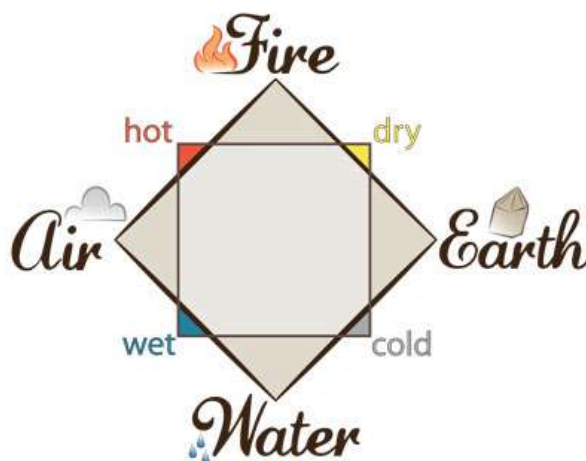
Figure 1-6. Aristotle's Four Elements and Four Properties
