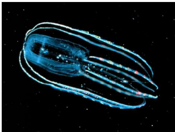
Figure 1-1. Bioluminescent Lobate Ctenophore (comb jellyfish)
