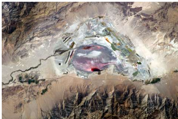
Figure 1-12. Owens Lake: A Mostly Dry Lake with Salt Deposits
