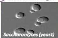
Saccharomyces (yeast)
