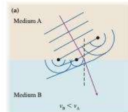
The wave travels farther on the right side in the less optically dense medium A than on the left side in denser medium B.
