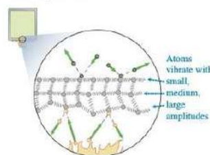
FIGURE 15.5 Microscopic view of a gas being heated by a flame.
