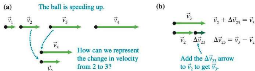
FIGURE 2.4 Determining the magnitude and direction of the velocity change arrow in a motion diagram.
