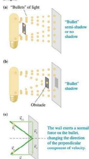
FIGURE 22.20 Newton's particle-bullet model of light.
