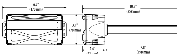
CDL Duct Mount
