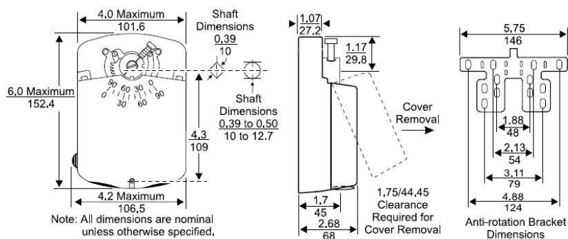
Dimensions, in./mm
