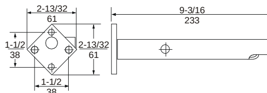
TE-6001-11 Duct Temperature Holder Dimensions, (in./mm)
