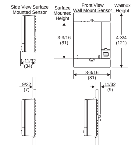
Wall Mount Humidity Transmitter Dimensions, in. (mm)
