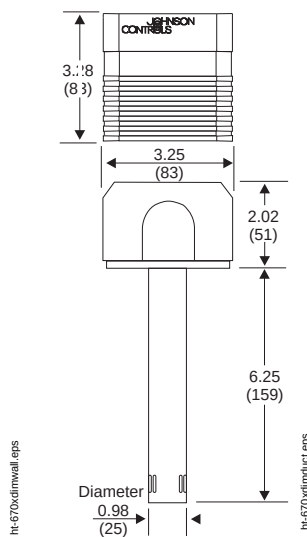
Duct Probe Humidity Transmitter Dimensions, in. (mm)
