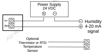
Room, Duct, OSA (RH or RH-T)
