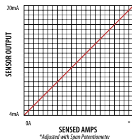
H221/321/421 LINEAR OUTPUT Scale software as shown
