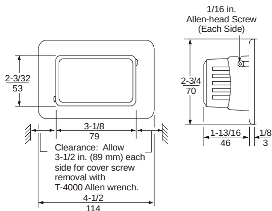
TE-6001-4 Temperature Element Holder Dimensions, (in./mm)
