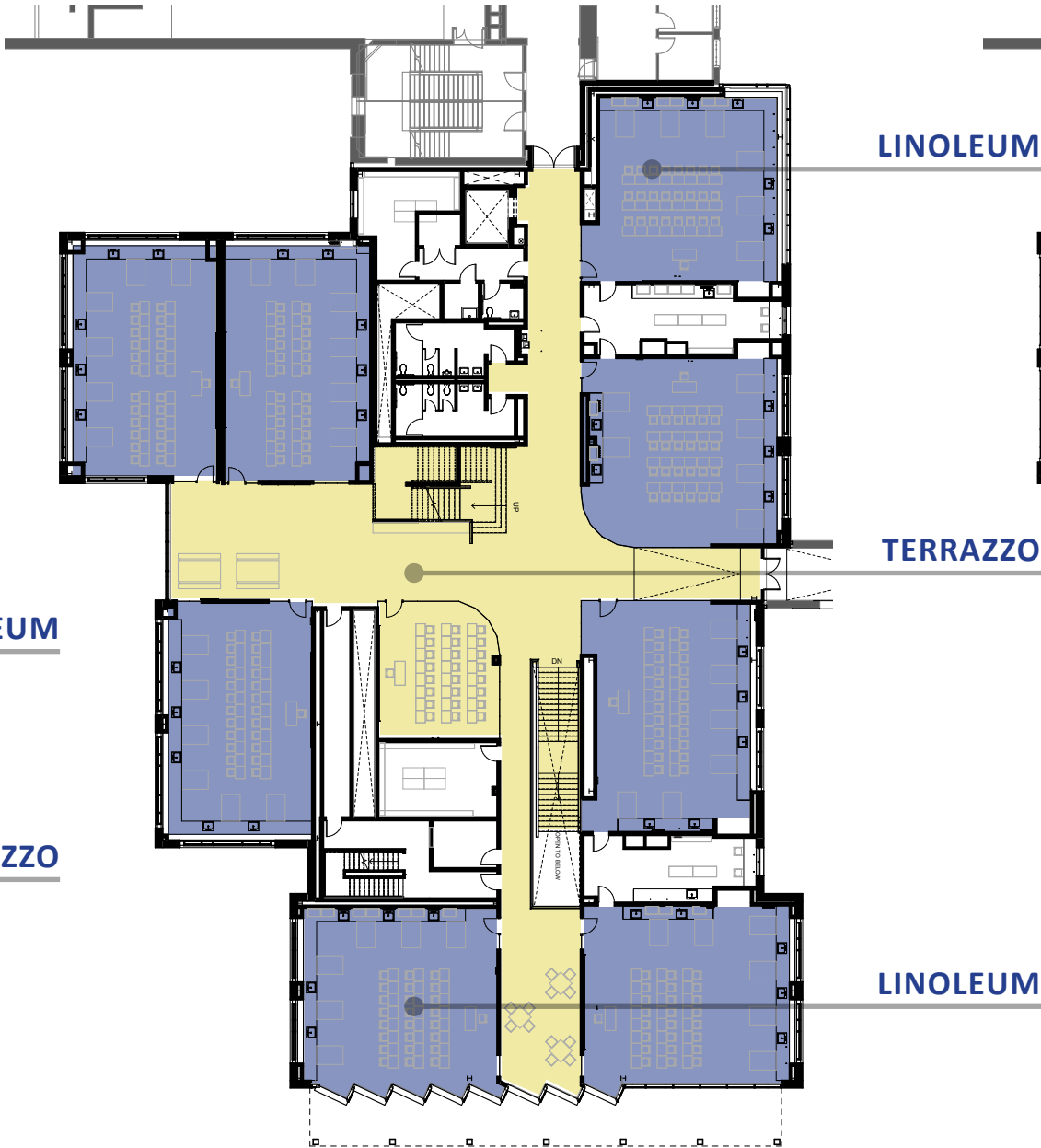
LEVEL 02 PLAN
