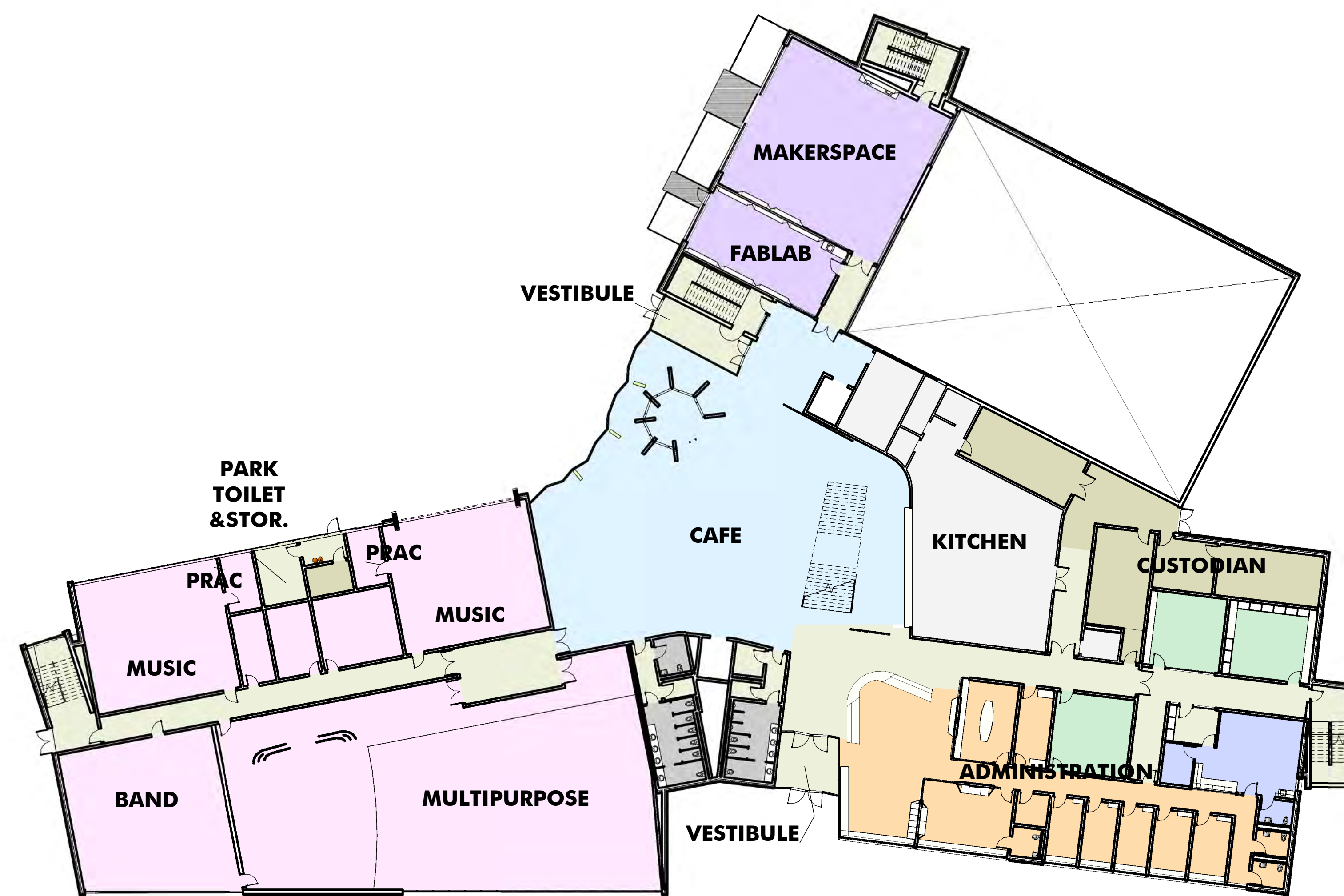
FIRST FLOOR
