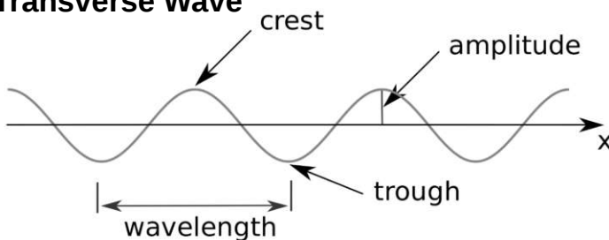
Transverse Wave
