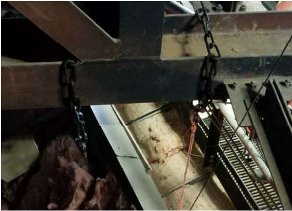
SPEAKER CLUSTER SHACKLES NOT MOUSED
