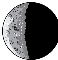
Mercury 0.38X
