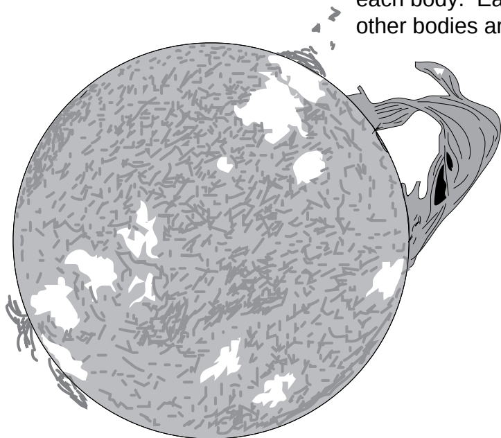
Sun 108X
