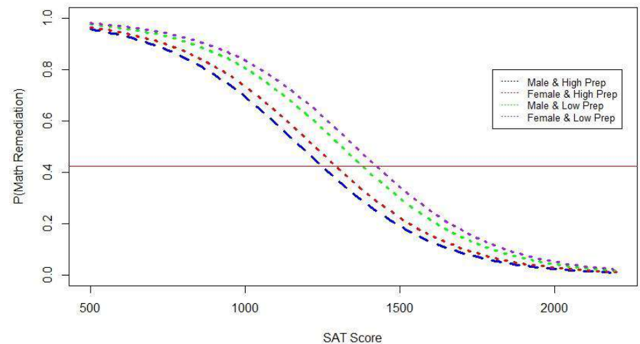
Probability of Math Remediation vs. SAT Score
