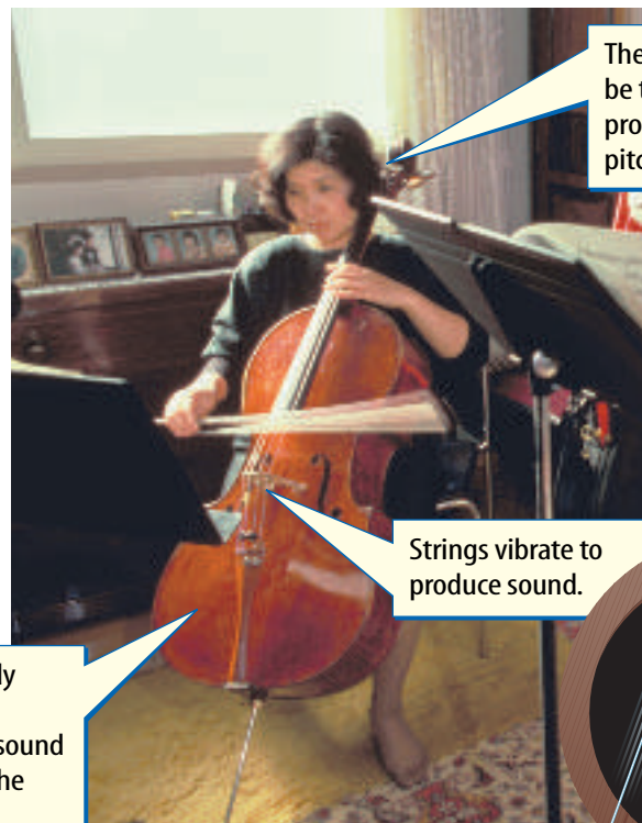
Figure 16 A cello is a stringed instrument. When strings vibrate, the natural frequencies of the instrument's body amplify the sound.
