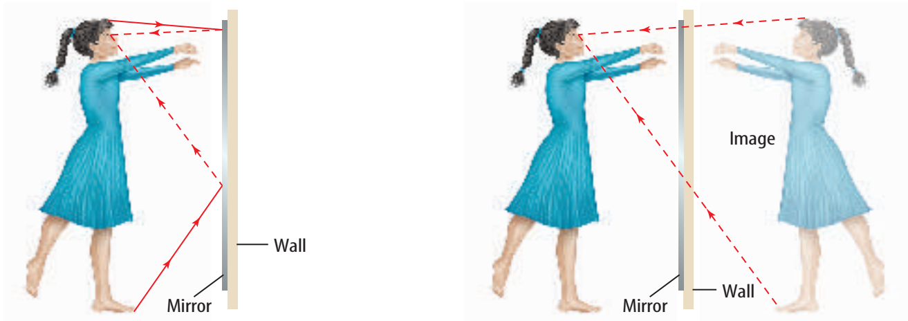
A Light rays that bounce off a person strike the mirror. Some of these light rays are reflected into the person's eye. B The light rays that are shown entering the person's eye seem to be coming from a person behind the mirror.
