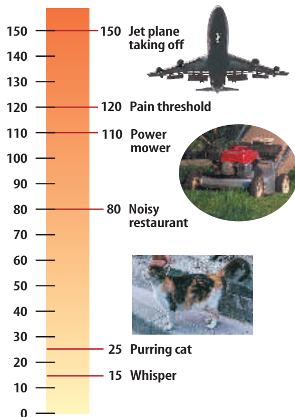
Figure 5 The loudness of sound is measured on the decibel scale.
