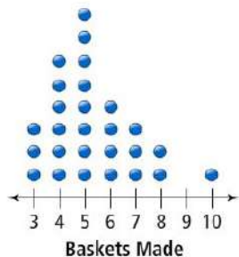
Dot Plot
