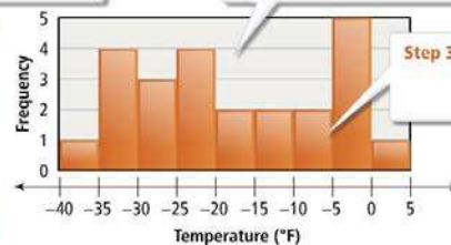
Histogram
