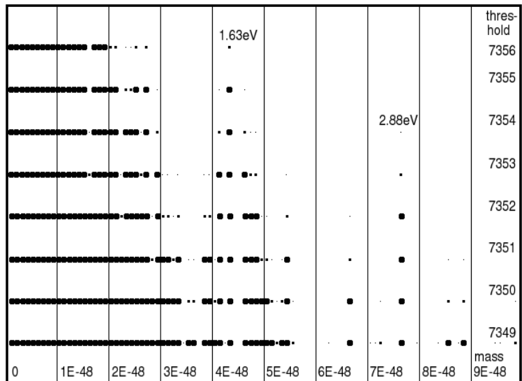
Figure 2: Tests for the electron neutrino, masses < 4 \text{ eV} . Initial radius 5, 99 values, 9 times piled (891 tests)
