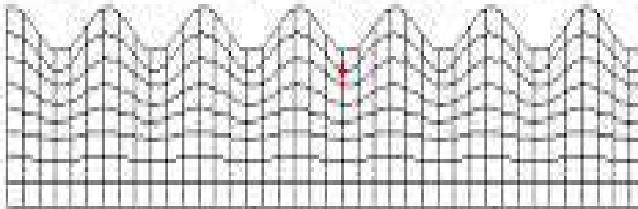
Surface Wave
