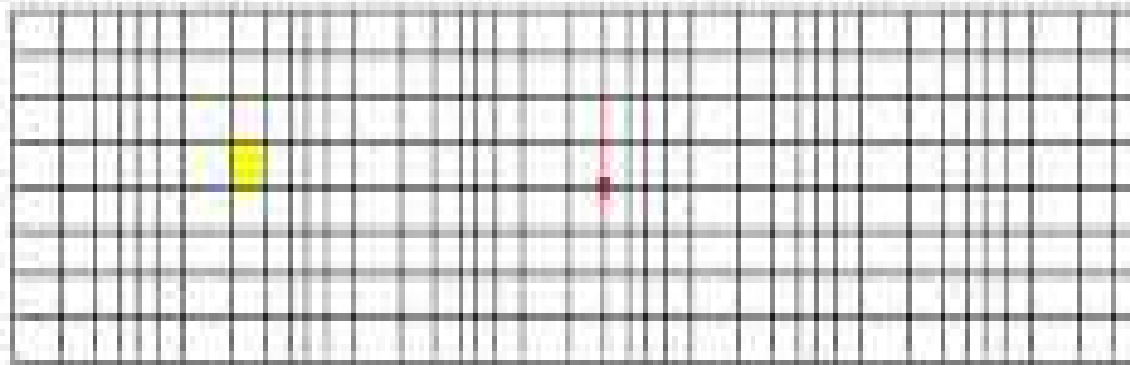
P-Wave
