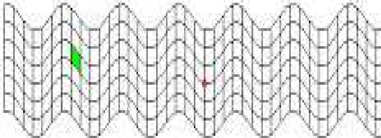
S-Wave
