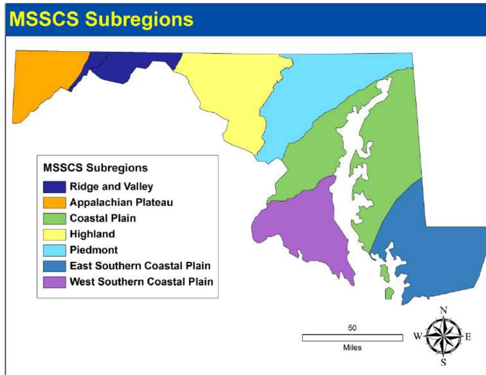
Figure 2-1. Map of the MSSCS subregions (Appalachian Region without Ridge and Valley included, Ridge and Valley, Eastern Southern Coastal Plain, and Western Southern Coastal Plain). The MSSCS regions discussed in this report are the combination of Appalachian Region (without Ridge and Valley) and Ridge and Valley into the “Appalachian Region” and combination of Eastern and Western subregions into the “Southern Coastal Plain region.”
