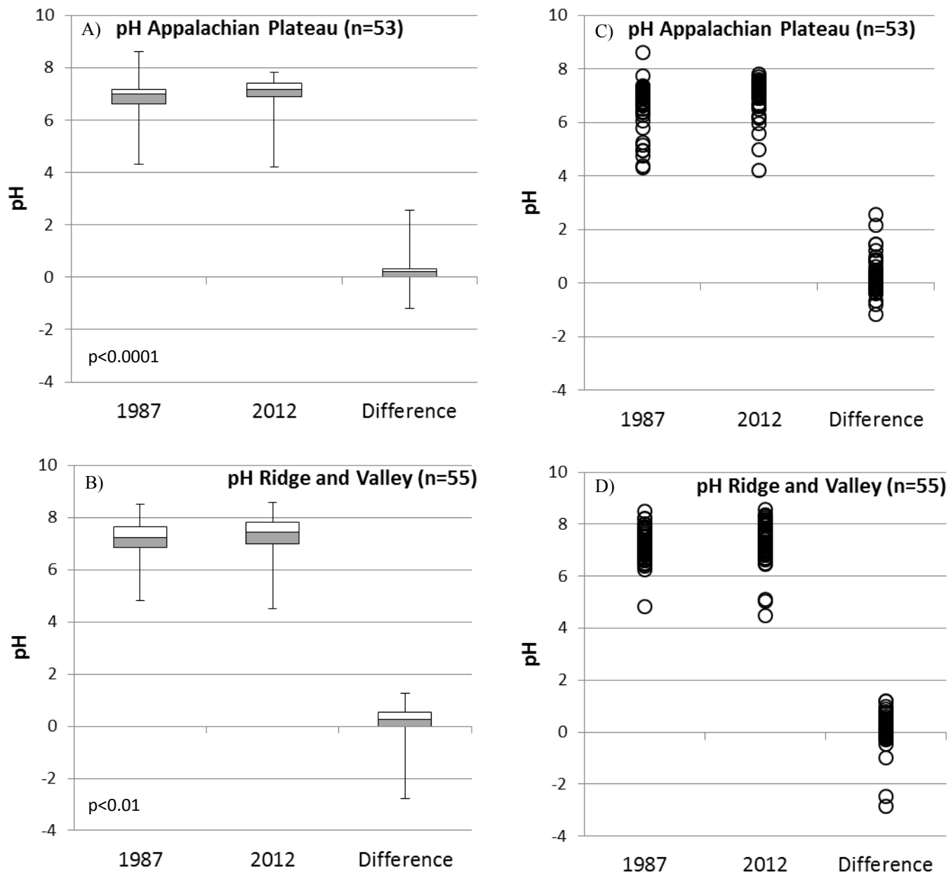
Figure 3-10. pH for the MSSCS subregions. Box and whisker plots for A) Appalachian Plateau and B) Ridge and Valley depict the 25th, 50th (median), and 75th percentile for 1987, 2012, and the difference between years. Whiskers indicate the minimum and maximum values in the dataset. P-values indicate significance from Wilcoxon Signed Rank test. Dot plots for C) Appalachian Plateau and D) Ridge and Valley show all values.
