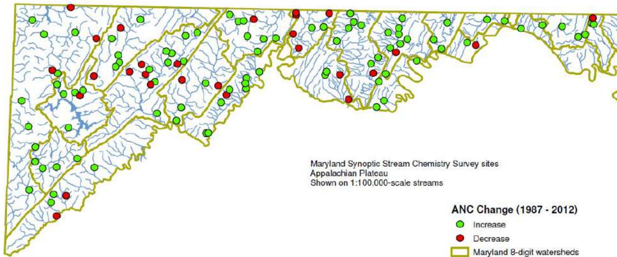
Figure 3-2. Map of the Appalachian Region showing whether site ANC increased or decreased between 1987 and 2012.
