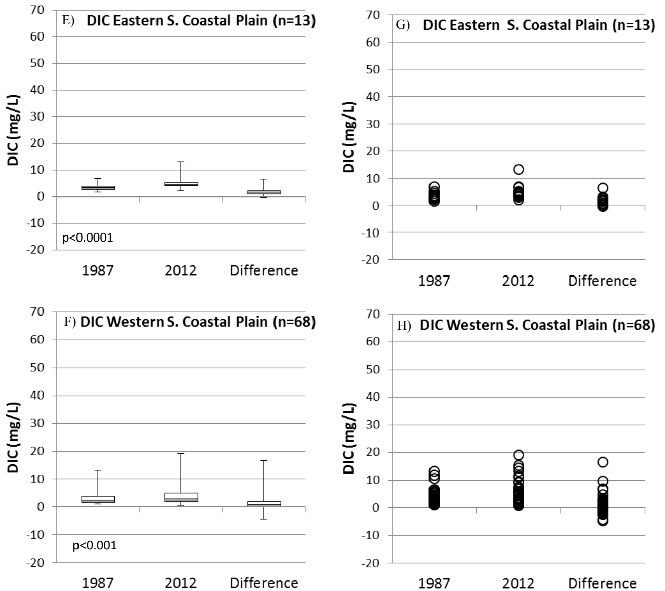
Figure 3 22 (Continued). Dissolved Inorganic Carbon (DIC) for the MSSCS subregions. Box and whisker plots for E) Eastern S. Coastal Plain and F) Western S. Coastal Plain depict the 25th, 50th (median), and 75th percentile for 1987, 2012, and the difference between years. Whiskers indicate the minimum and maximum values in the dataset. P-values indicate significance from Wilcoxon Signed Rank test.
