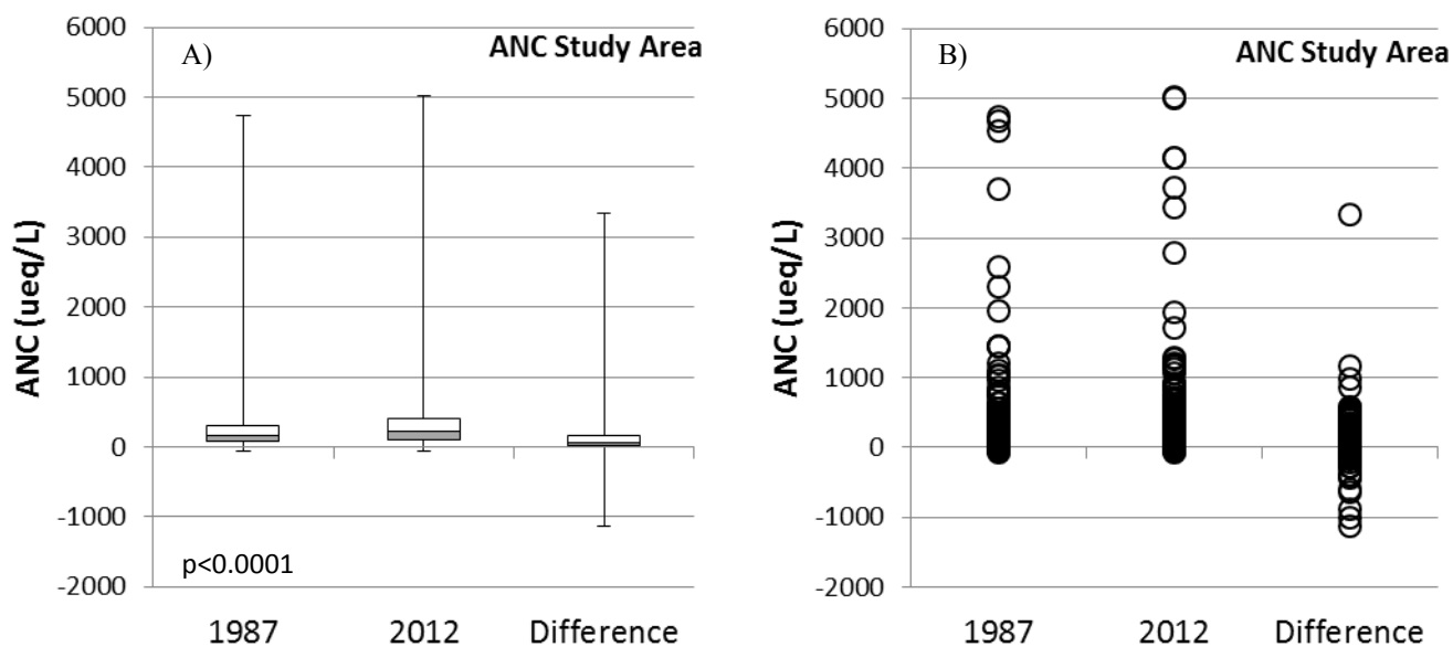
Figure 3-4. Acid neutralizing capacity (ANC) in the study area. Panel A) Box and whisker plot depicting the 25 th , 50 th (median), and 75 th percentile for 1987, 2012, and the difference between years. Whiskers indicate the minimum and maximum values in the dataset. P-values indicate significance from Wilcoxon Signed Rank test. Panel B) Dot plot showing all values.
