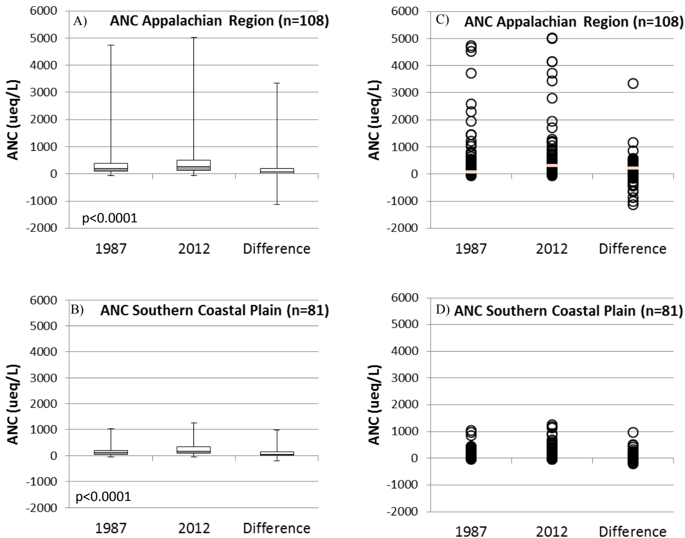
Figure 3-5. Acid neutralizing capacity (ANC) in Appalachian Region and Southern Coastal Plain. Box and whisker plots for A) Appalachian Region and B) Southern Coastal Plain depict the 25 th , 50 th (median), and 75 th percentile for 1987, 2012, and the difference between years. Whiskers indicate the minimum and maximum values in the dataset. P-values indicate significance from Wilcoxon Signed Rank test. Dot plots for C) Appalachian Region and D) Southern Coastal Plain show all values.
