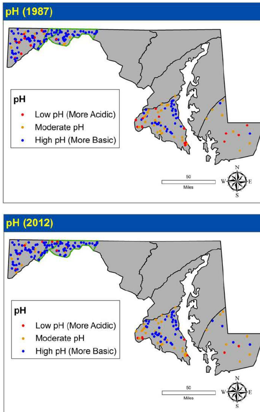
Figure 3-7. Maps showing the pH for each site. Top Panel shows Round 1 (1987) and Bottom Panel shows Round 2 (2012) of MSSCS. The region outlined in green contains the
