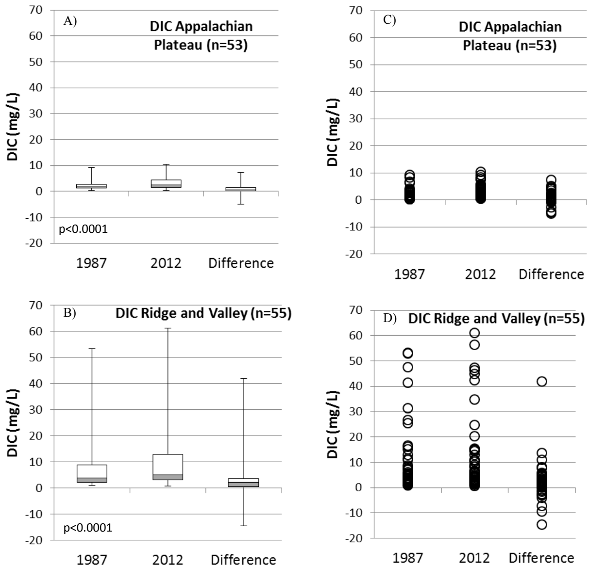
Figure 3-22. Dissolved Inorganic Carbon (DIC) for the MSSCS subregions. Box and whisker plots for A) Appalachian Plateau and B) Ridge and Valley depict the 25th, 50th (median), and 75th percentile for 1987, 2012, and the difference between years. Whiskers indicate the minimum and maximum values in the dataset. P-values indicate significance from Wilcoxon Signed Rank test. Dot plots for C) Appalachian Plateau and D) Ridge and Valley show all values.
