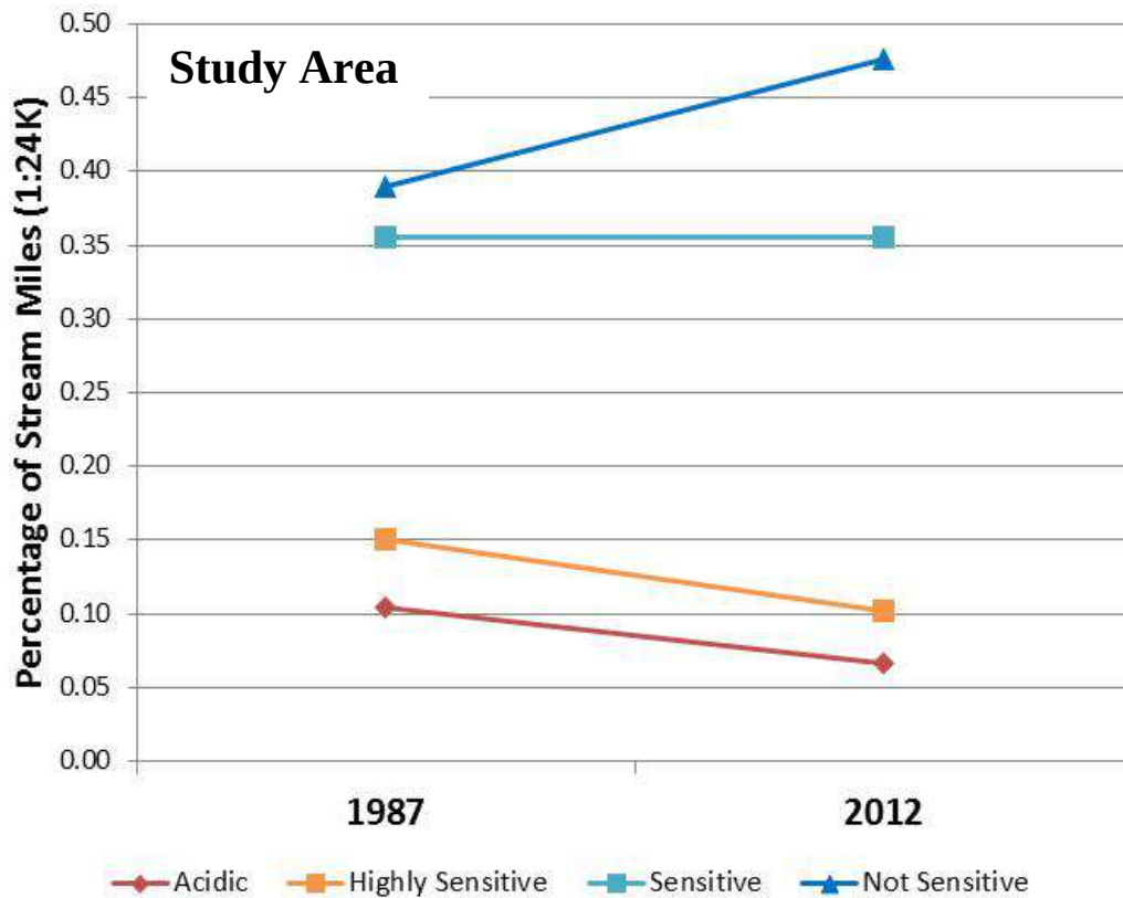
Figure 3-23. The percentage of stream miles in each of the four ANC categories for 1987 and 2012
