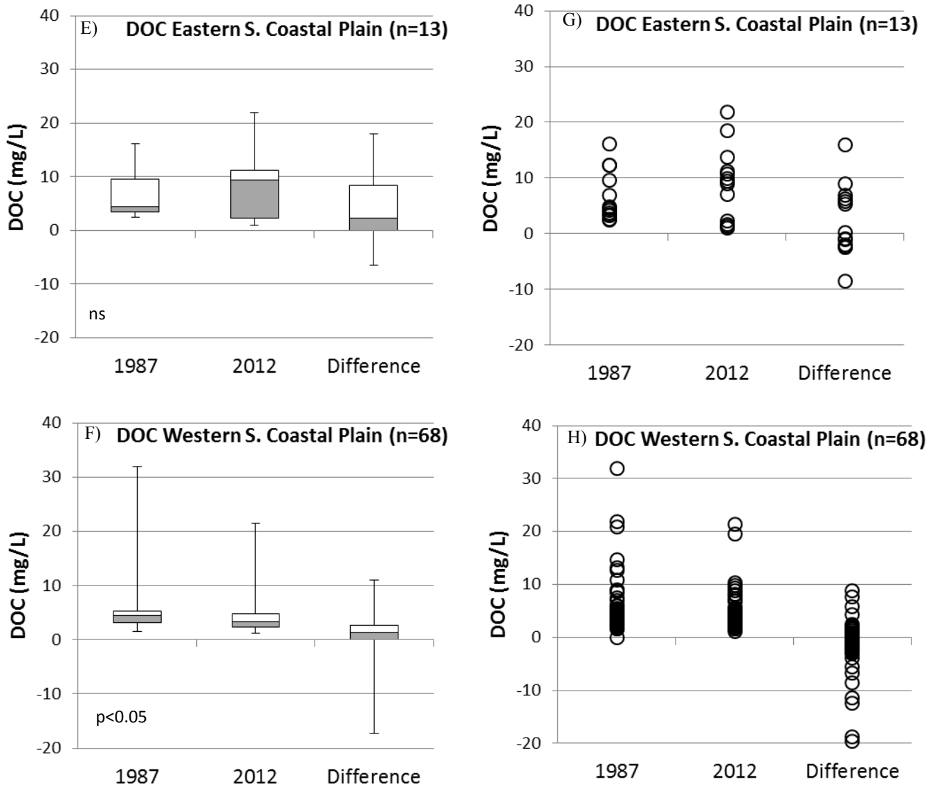
Figure 3 18 (Continued). Dissolved Organic Carbon (DOC) for the MSSCS subregions. Box and whisker plots for E) Eastern S. Coastal Plain and F) Western S. Coastal Plain depict the 25th, 50th (median), and 75th percentile for 1987, 2012, and the difference between years. Whiskers indicate the minimum and maximum values in the dataset. P-values indicate significance from Wilcoxon Signed Rank test. Dot plots for G) Eastern S. Coastal Plain and H) Western S. Coastal Plain show all values.
