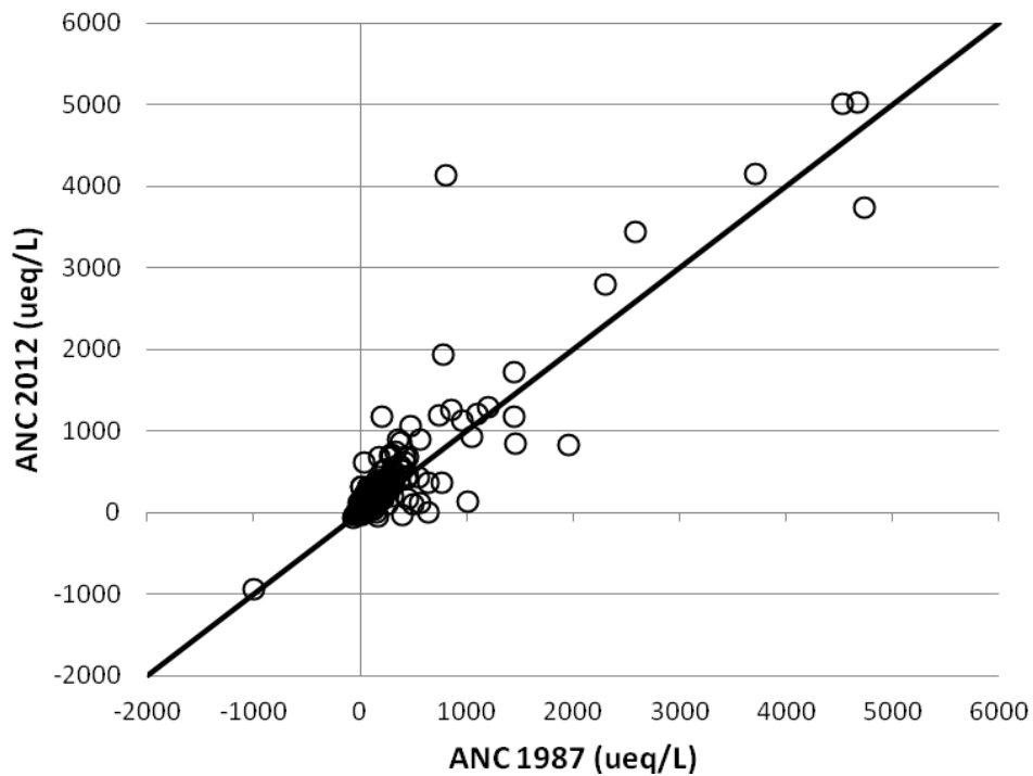
Figure 3-5. Scatterplot of acid neutralizing capacity (ANC) comparing the values at all individual sites within the study area in 1987 vs. 2012. A 1:1 line is drawn to indicate no change between years. Sites falling above this line had an increase in ANC between years and those falling below this line had a decrease in ANC between years.
