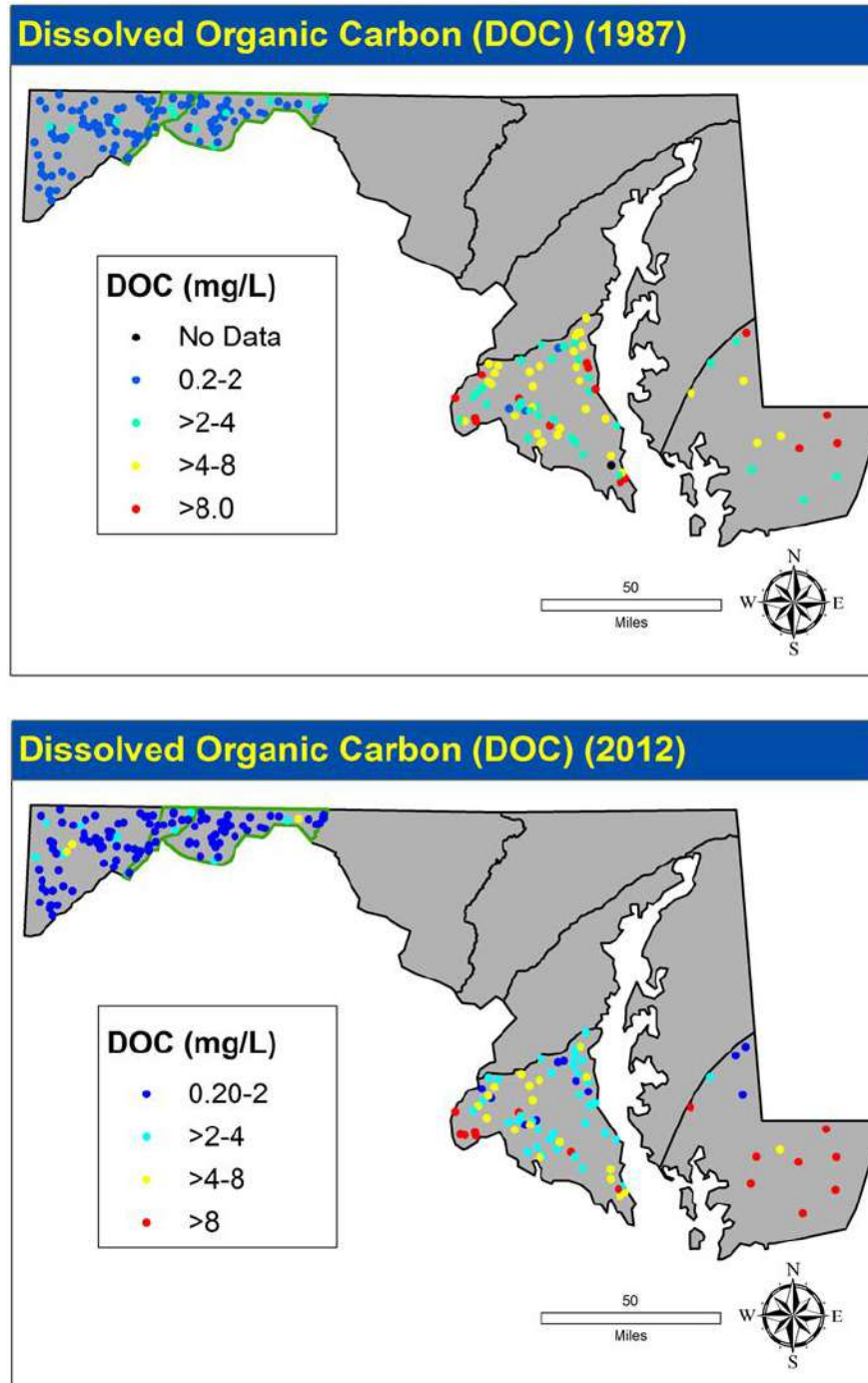
Figure 3-15. Maps showing the dissolved organic carbon (DOC) (mg/L) for each site. Top Panel shows Round 1 (1987) and Bottom Panel shows Round2 (2012) of MSSCS. The region outlined in green contains the Ridge and Valley MSSCS subregion.
