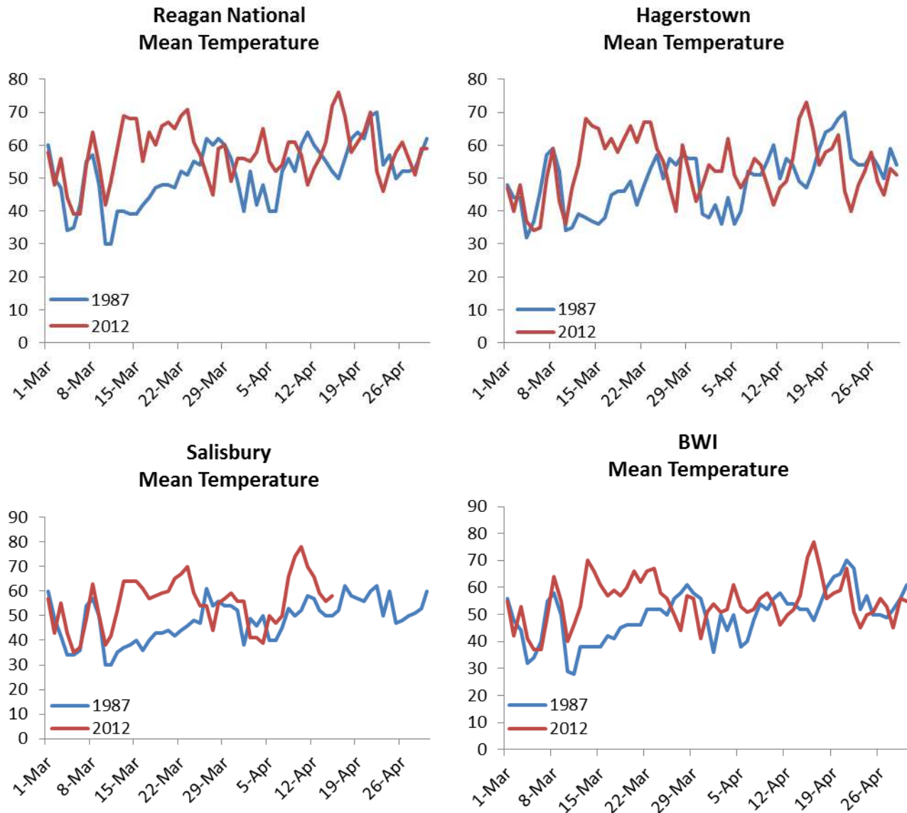
Figure C-1. Mean Temperature (degrees F) within the MSSCS sampling extent. Upper Left Panel: Reagan National Airport. Upper Right Panel: Hagerstown Airport. Lower Left Panel: Salisbury Airport. Lower Right Panel: Baltimore-Washington International Airport.
