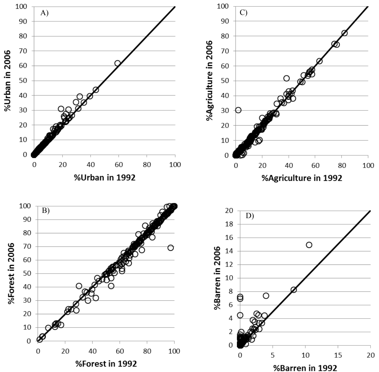
Figure B-8. Scatterplots of land use comparing the percentage of each land use type in 1992 and 2006. A) Urban, B) Forest, C) Agriculture, D) Barren, E) Water, and F) Wetland. A 1:1 line is drawn on each figure to indicate no change. Points falling above this line showed an increase in the land use type between years and points falling below the line showed a decrease in the land use type between years.
