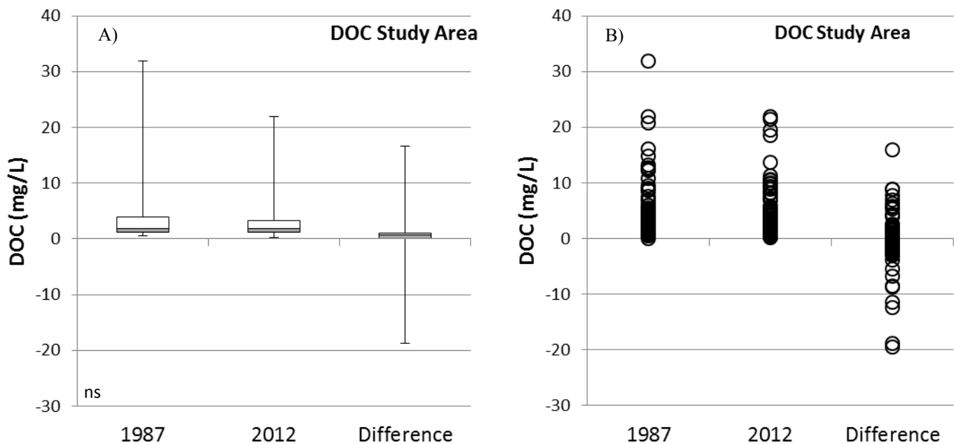
Figure 3-16. Dissolved Organic Carbon (DOC) in the study area. Panel A) Box and whisker plot depicting the 25 th , 50 th (median), and 75 th percentile for 1987, 2012, and the difference between years. Whiskers indicate the minimum and maximum values in the dataset. ns indicates no significant difference from Wilcoxon Signed Rank test. Panel B) Dot plot showing all values.
