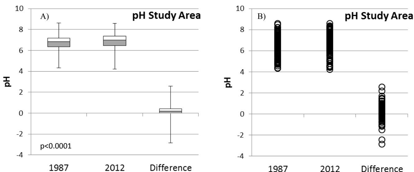
Figure 3-8. pH in the study area. Panel A) Box and whisker plot depicting the 25 th , 50 th (median), and 75 th percentile for 1987, 2012, and the difference between years. Whiskers indicate the minimum and maximum values in the dataset. P-values indicate significance from Wilcoxon Signed Rank test. Panel B) Dot plot showing all values.
