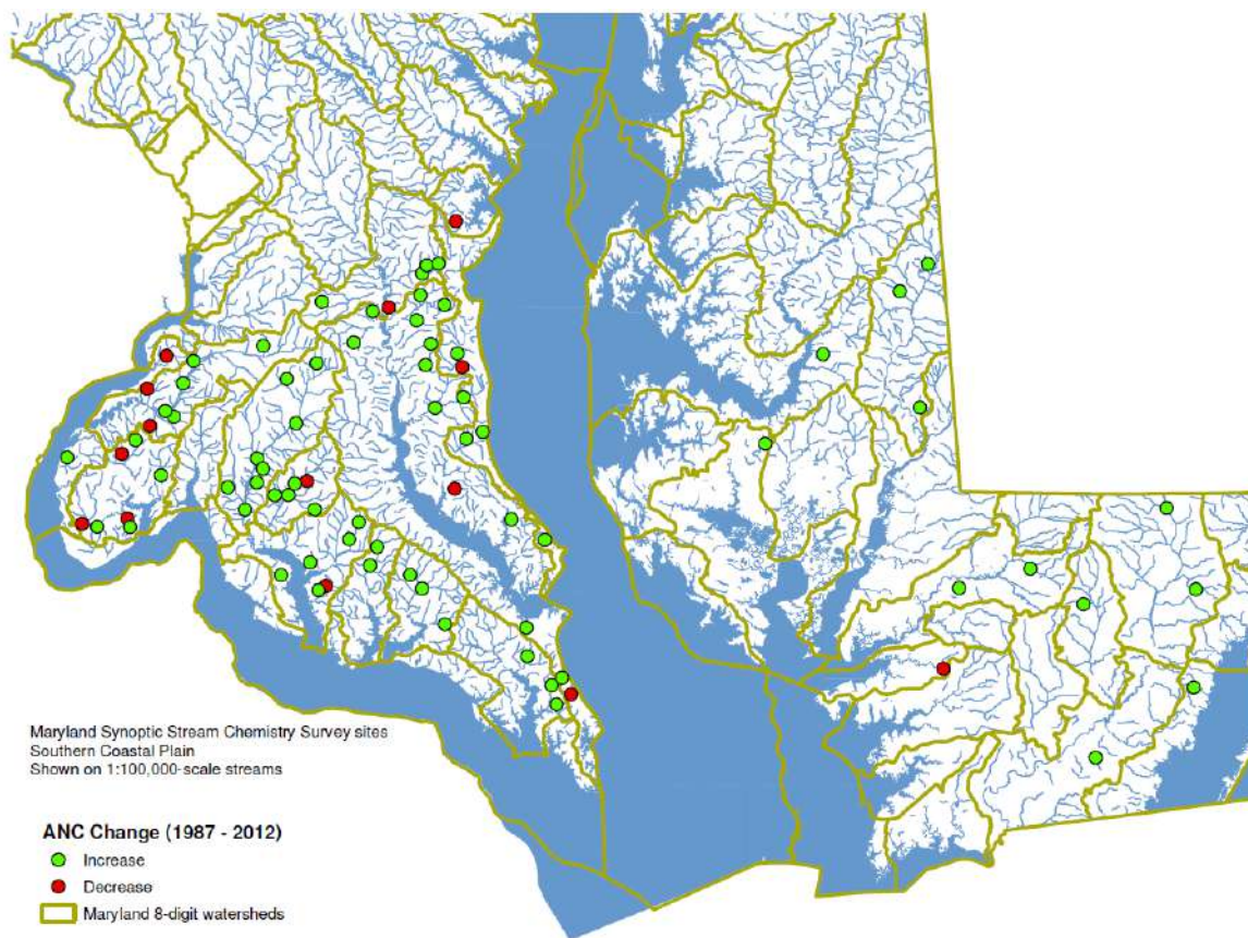
Figure 3-3. Map of the Coastal Plain showing whether site ANC increased or decreased between 1987 and 2012.
