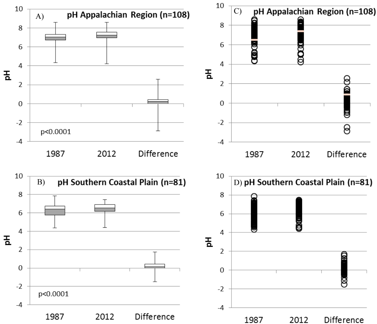
Figure 3-9. pH in MSSCS Regions. Box and whisker plots for A) Appalachian Region and B) Southern Coastal Plain depict the 25th, 50th (median), and 75th percentile for 1987, 2012, and the difference between years. Whiskers indicate the minimum and maximum values in the dataset. P-values indicate significance from Wilcoxon Signed Rank test. Dot plots for C) Appalachian Region and D) Southern Coastal Plain show all values.
