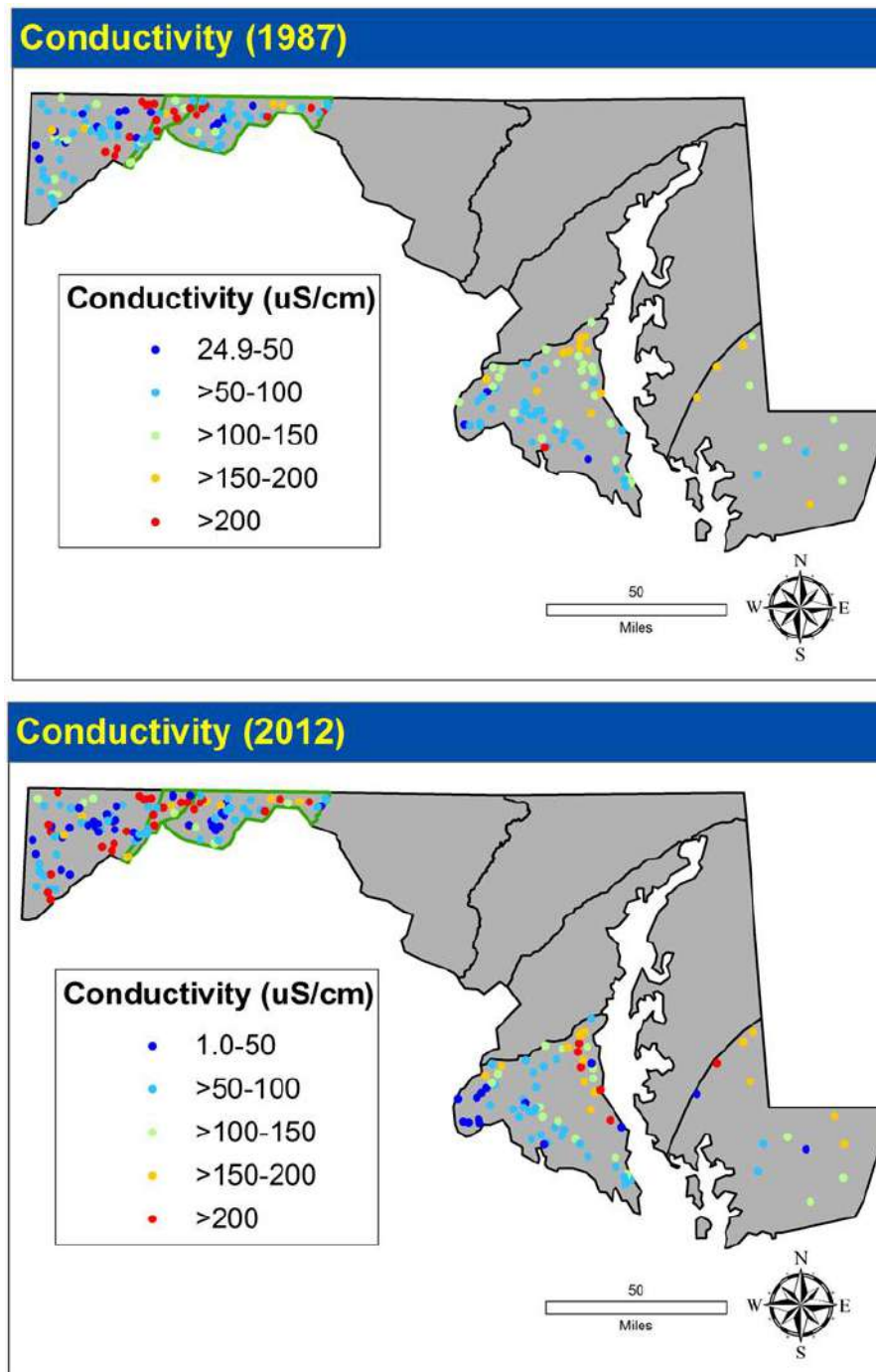
Figure 3-11. Maps showing the conductivity ( \mu\text{S}/\text{cm} ) category for each site. Top Panel shows Round 1 (1987) and Bottom Panel shows Round2 (2012) of MSSCS. The region
