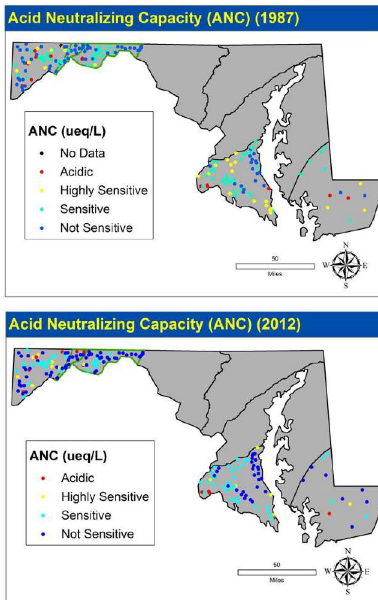
Figure 3-1. Maps showing the ANC category for each site. Top panel shows Round 1 (1987) and bottom panel shows Round2 (2012) of MSSCS. The area outlined in green contains the Ridge and Valley MSSCS subregion. See Table 1-2 for the ANC values that bound each category.
