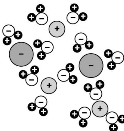
NaCl in Water
