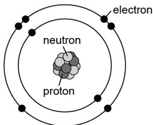
Bohr Model of an Oxygen Atom
