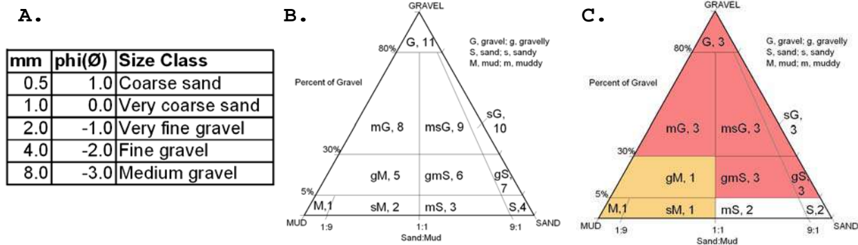
Figure 1. The grain size scales available in the grain size dataset. A.) A portion of the full phi scale used in the dataset. B.) The Folk classification with 12 classes. The text code is followed by the numeric code assigned in the dataset; anything larger than gravel is Hard, 12. C.) The Folk classification with four classes; anything larger than gravel is Hard, 4. The colors identify different Folk text codes that were given the same numeric code in the dataset.
