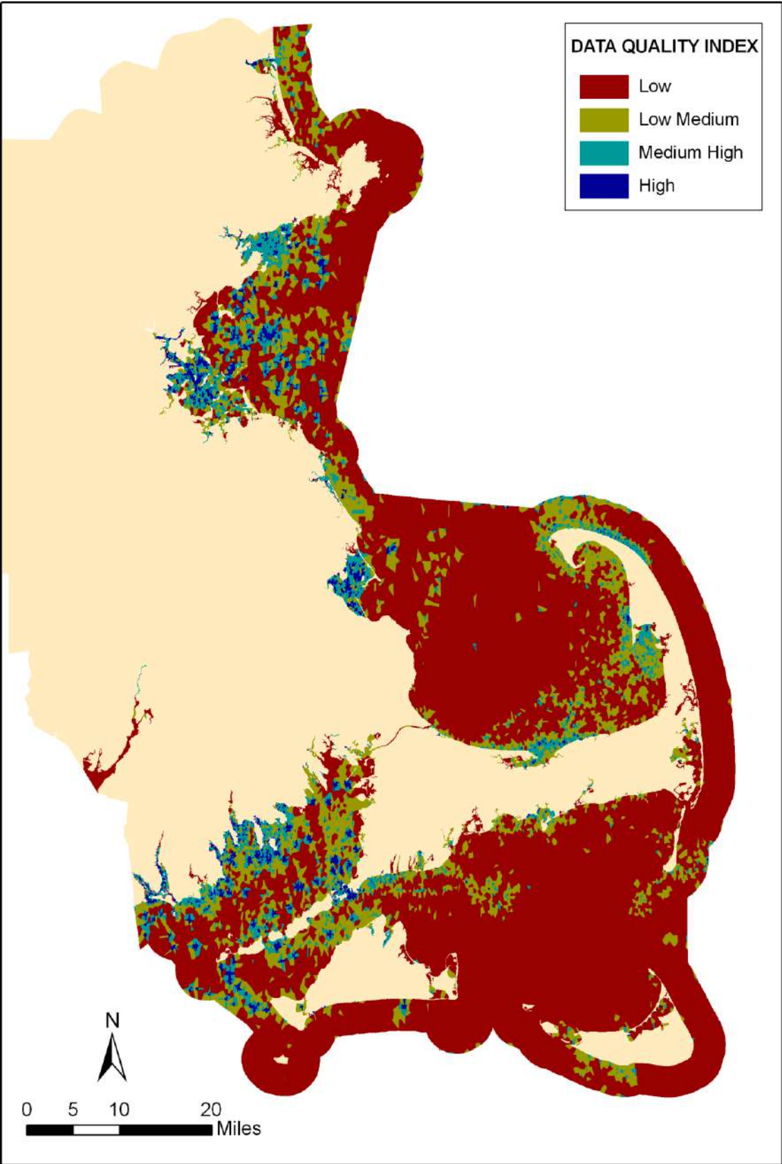
Figure 6. Spatial distribution of the quality assessment index combining data quality and density. Red=low quality (1 st quantile), mustard=low-medium quality (2 nd quantile), teal=medium-high quality (3 rd quantile), and blue= high quality (4 th quantile).
