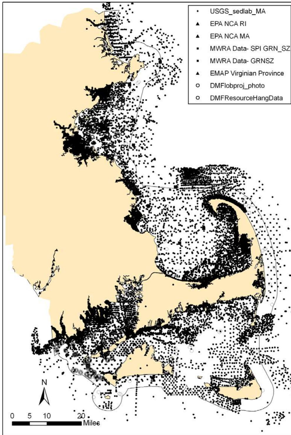
Figure 2. Surficial sediment points in Massachusetts and vicinity. A) usSEABED datapoints, B) additional datasets.
