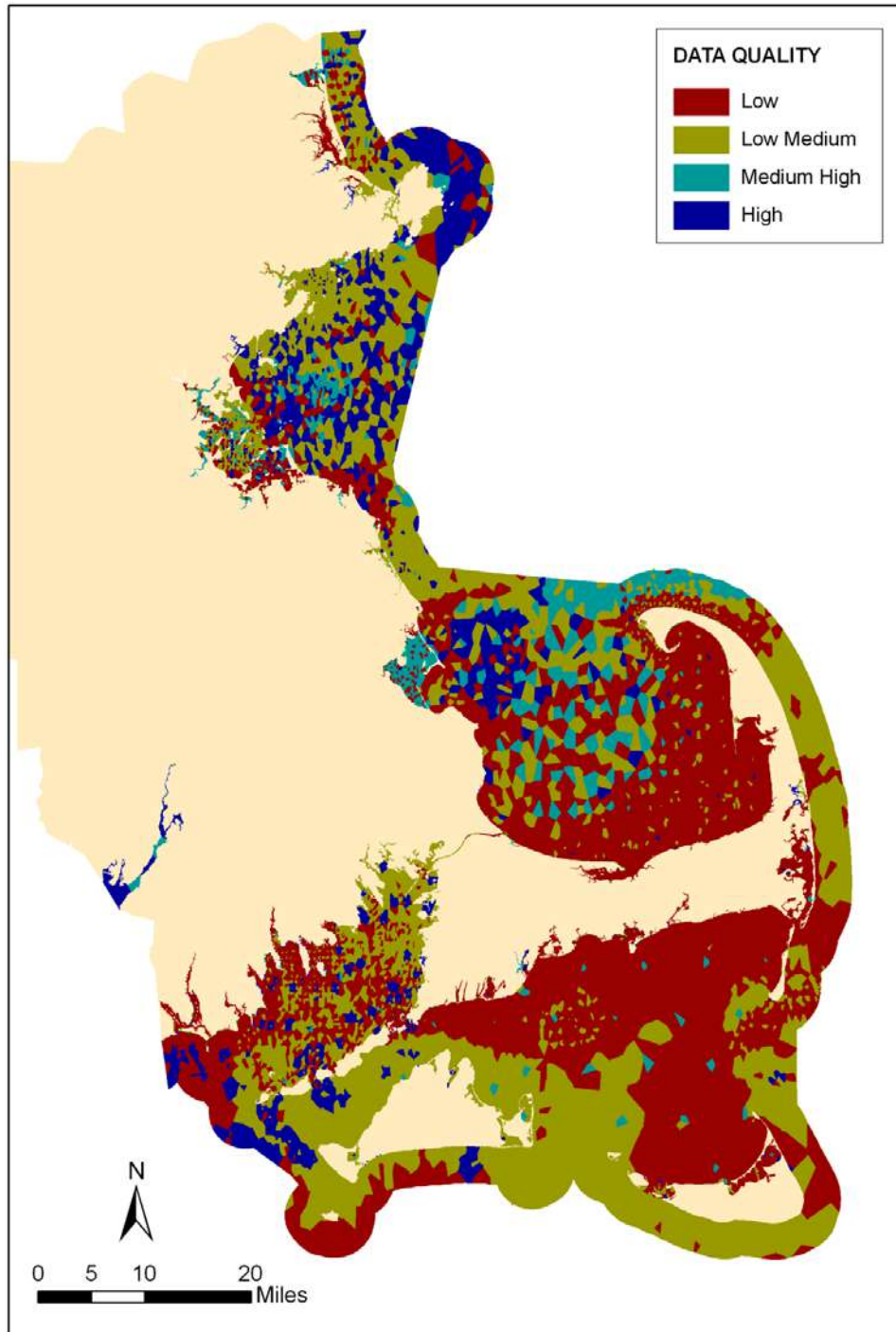
Figure 5. Spatial distribution of data quality. Red=low quality (1.00-1.99), mustard=low-medium quality (2.00-2.99), teal=medium-high quality (3.00-3.99), and blue=high quality (4.00-4.99).
