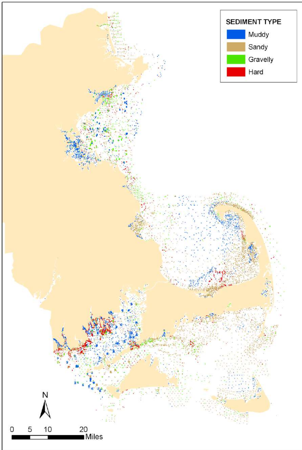
Figure 4A. Sediment distribution map gridded with 250 m 2 grid cells and B) Thiessen polygon interpolation. Blue=muddy sediment, brown=sandy sediment, green=gravelly sediment, and red=hard sediment.
