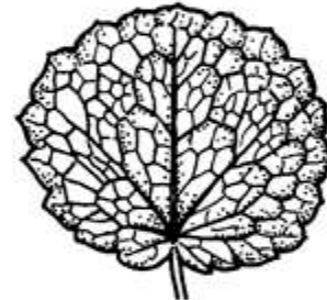
RETICULATE
