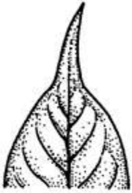
CAUDATE
