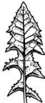
RUNCINATE
