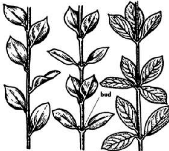
ALTERNATE
