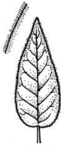
CILIATE
