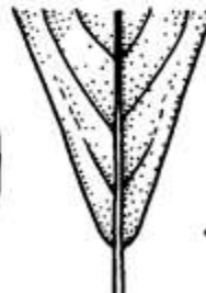
CUNEATE
