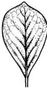
OBOVATE
