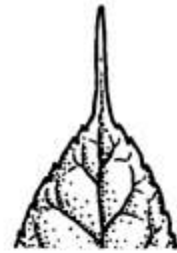
ARISTATE
