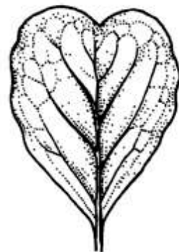
OBOVATE
