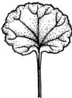
RENIFORM
