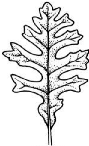
CLEFT
