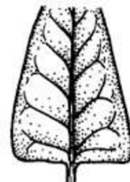
TRUNCATE
