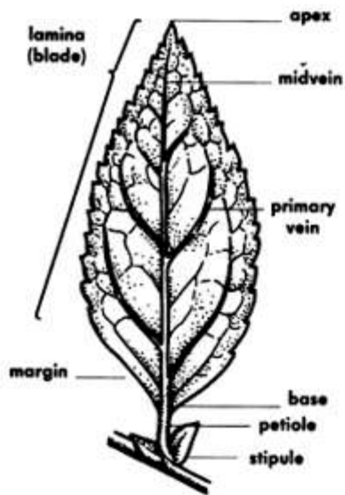
LEAF PARTS
