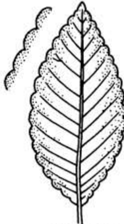
CRENATE
