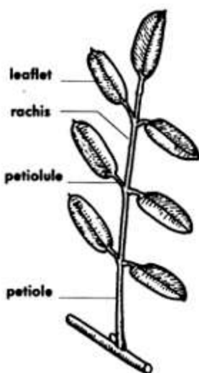
ODD-PINNATE
